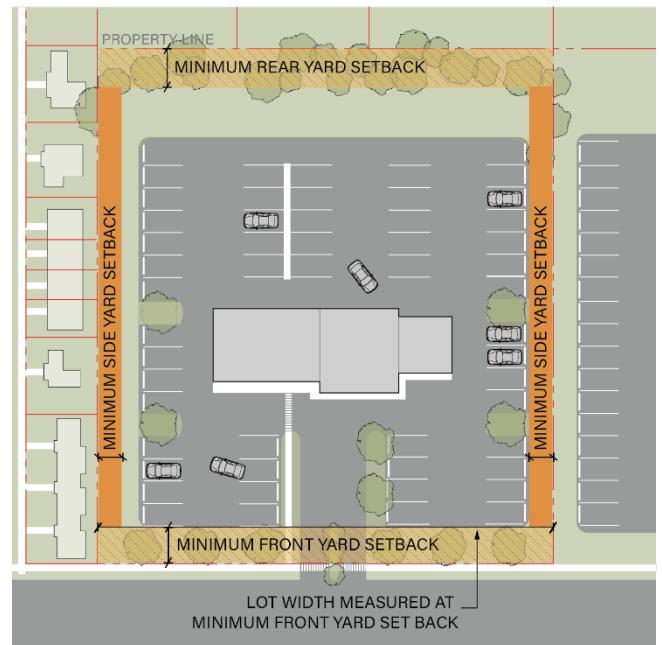
Example of minimum setback and lot width measurements
