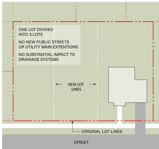
Example of minor subdivision
