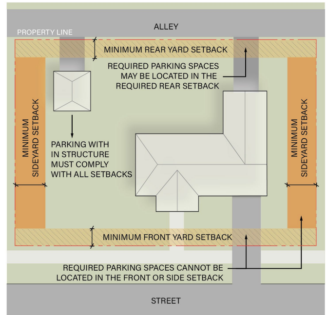
Example of single-family and two-family residential parking locations
