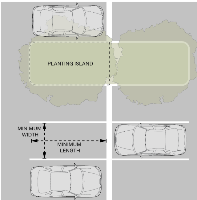
Example of parking stall dimensions
