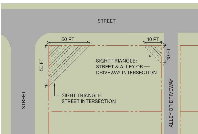
Example of sight triangle measurement
